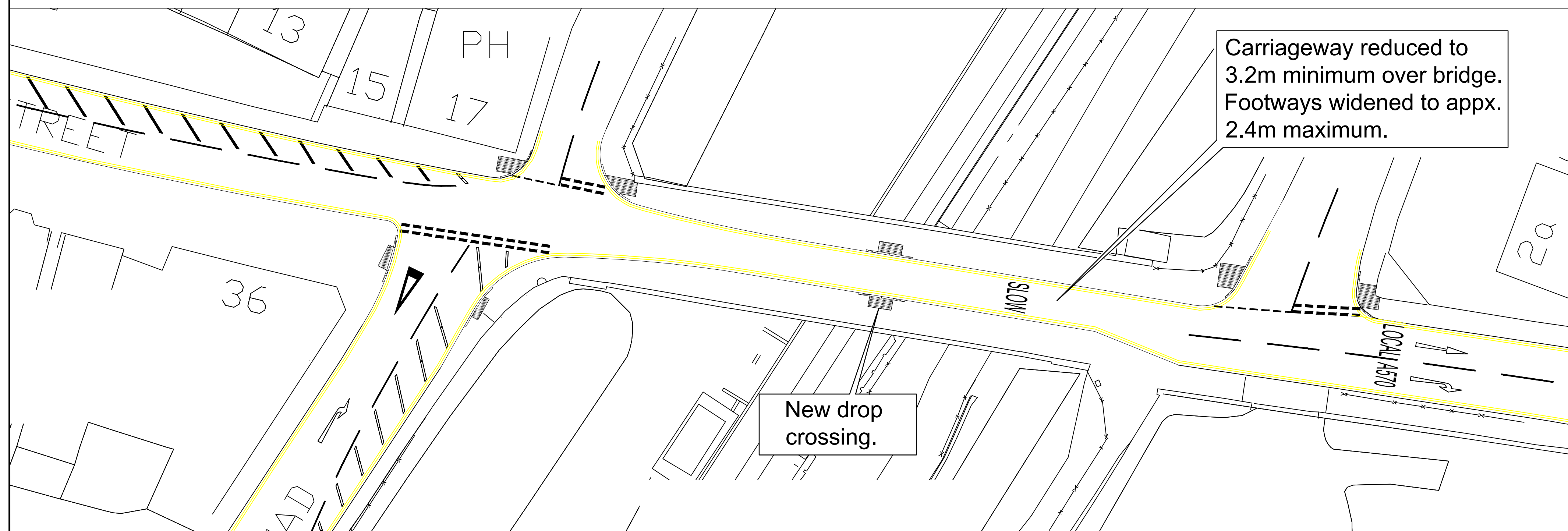
Derby Street Railway Bridge - Scale 1:200
