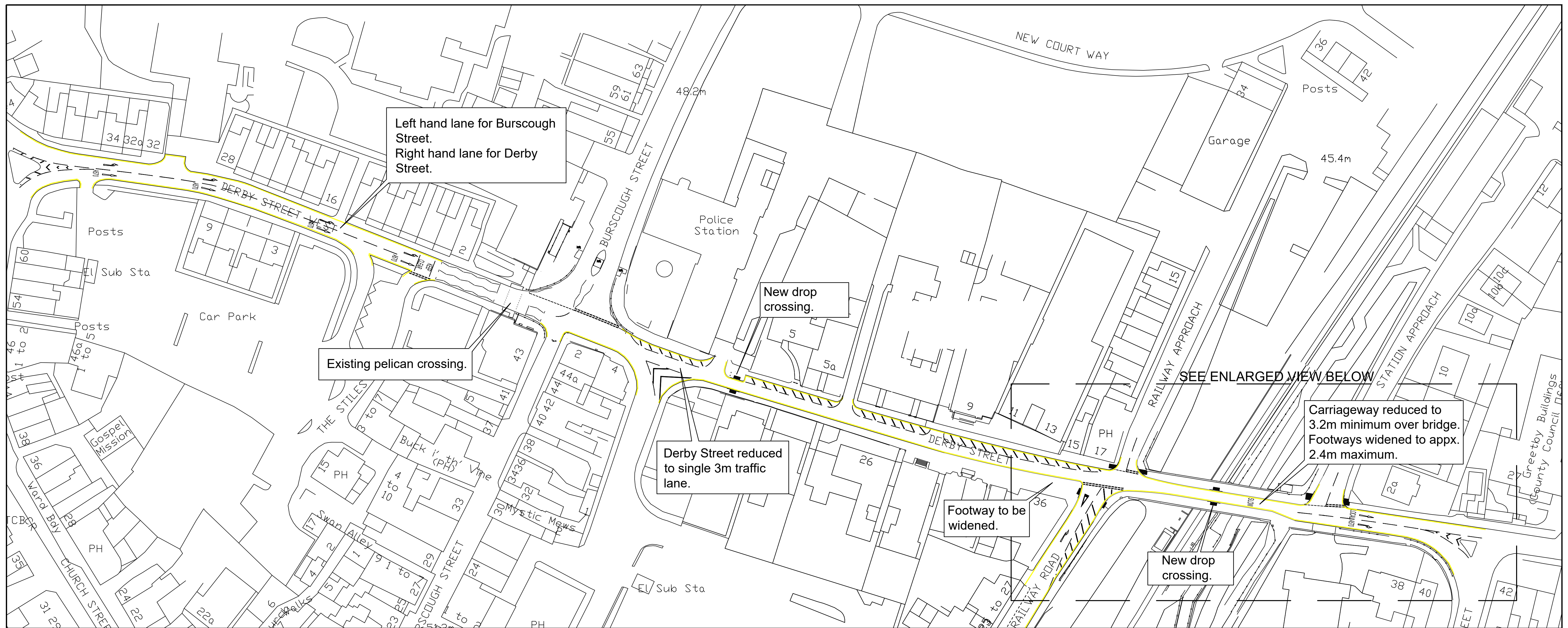
General Layout - Scale 1:500
